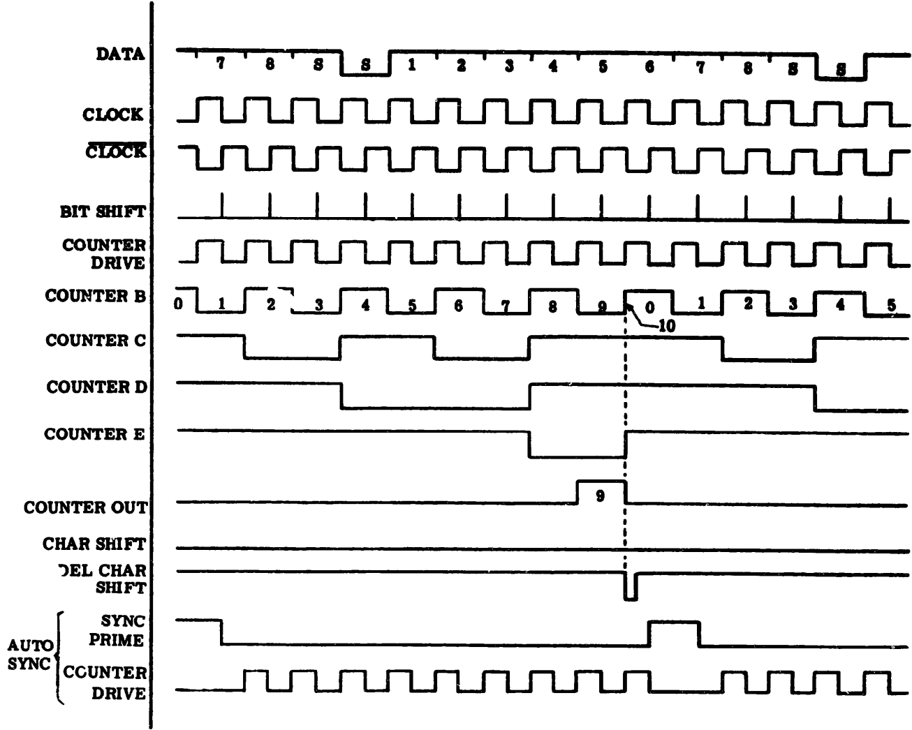
Figure 17- RD Logic for 10 Units, 5-Level (Start-Stop)
