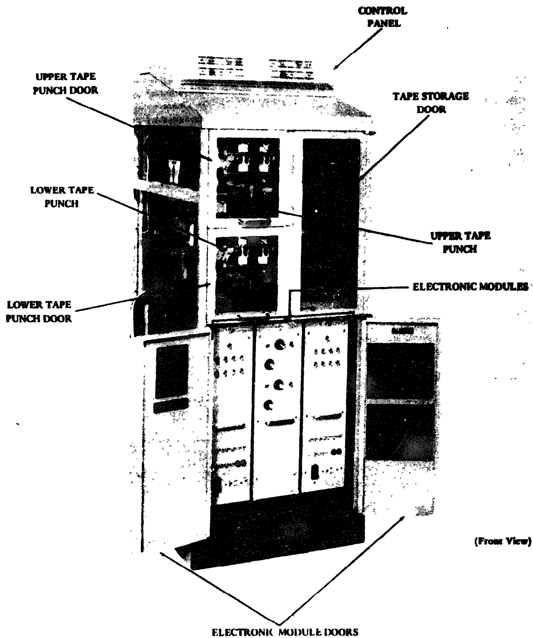
Figure 1 Receiver Cabinet
