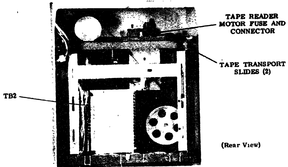
Figure 7- Tape Transport
