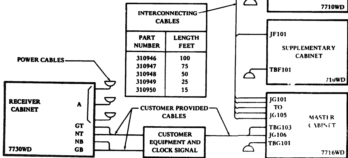
Figure 10- Interconnecting Cabling Diagram
