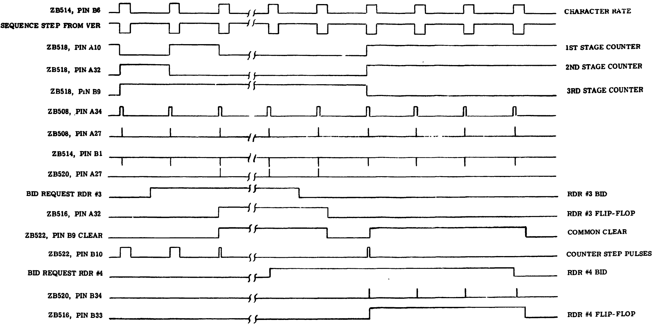
Figure 11- Timing Diagram For Sequence Control
