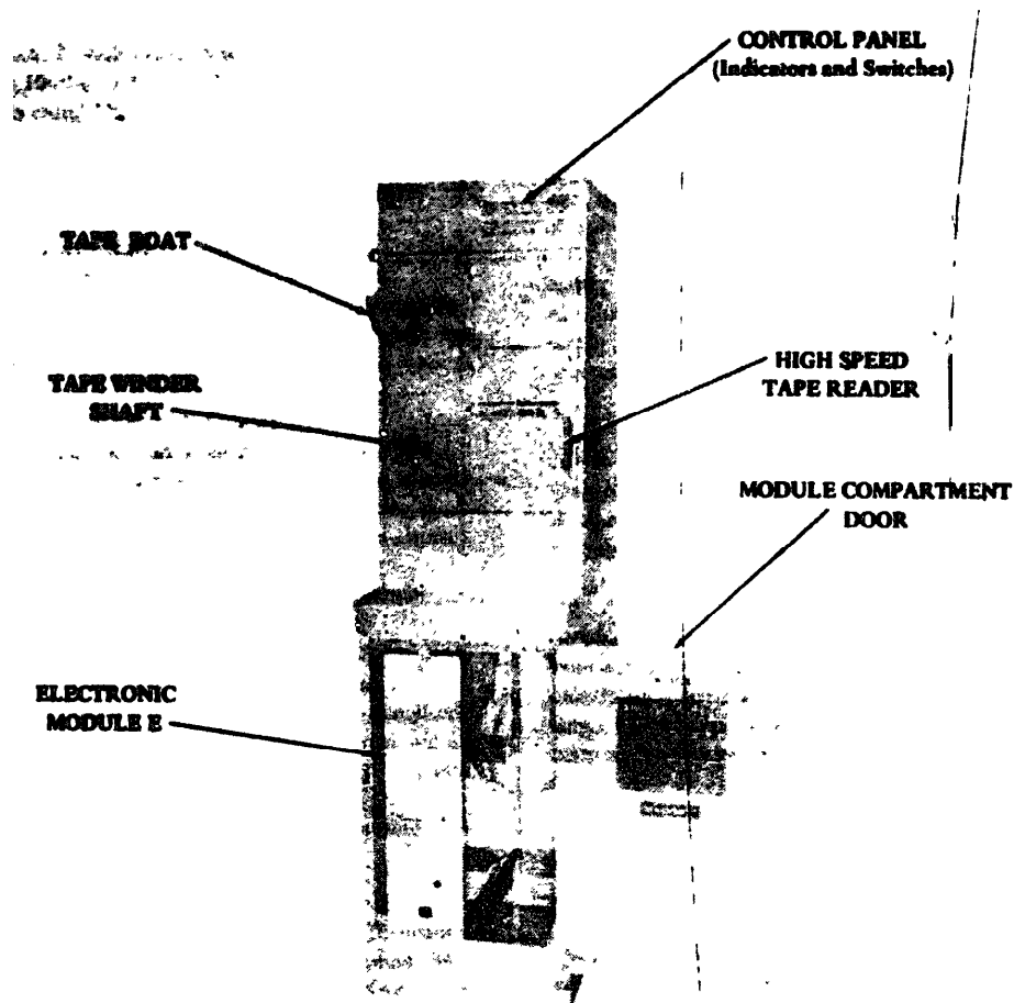
Figure 2- Supplementary High Speed Tape Sender
