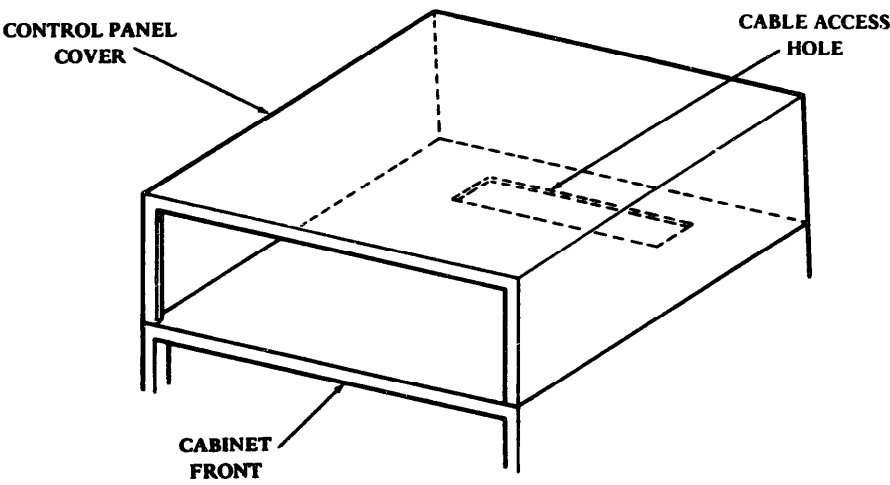
Figure 4- Cable Access Hole
